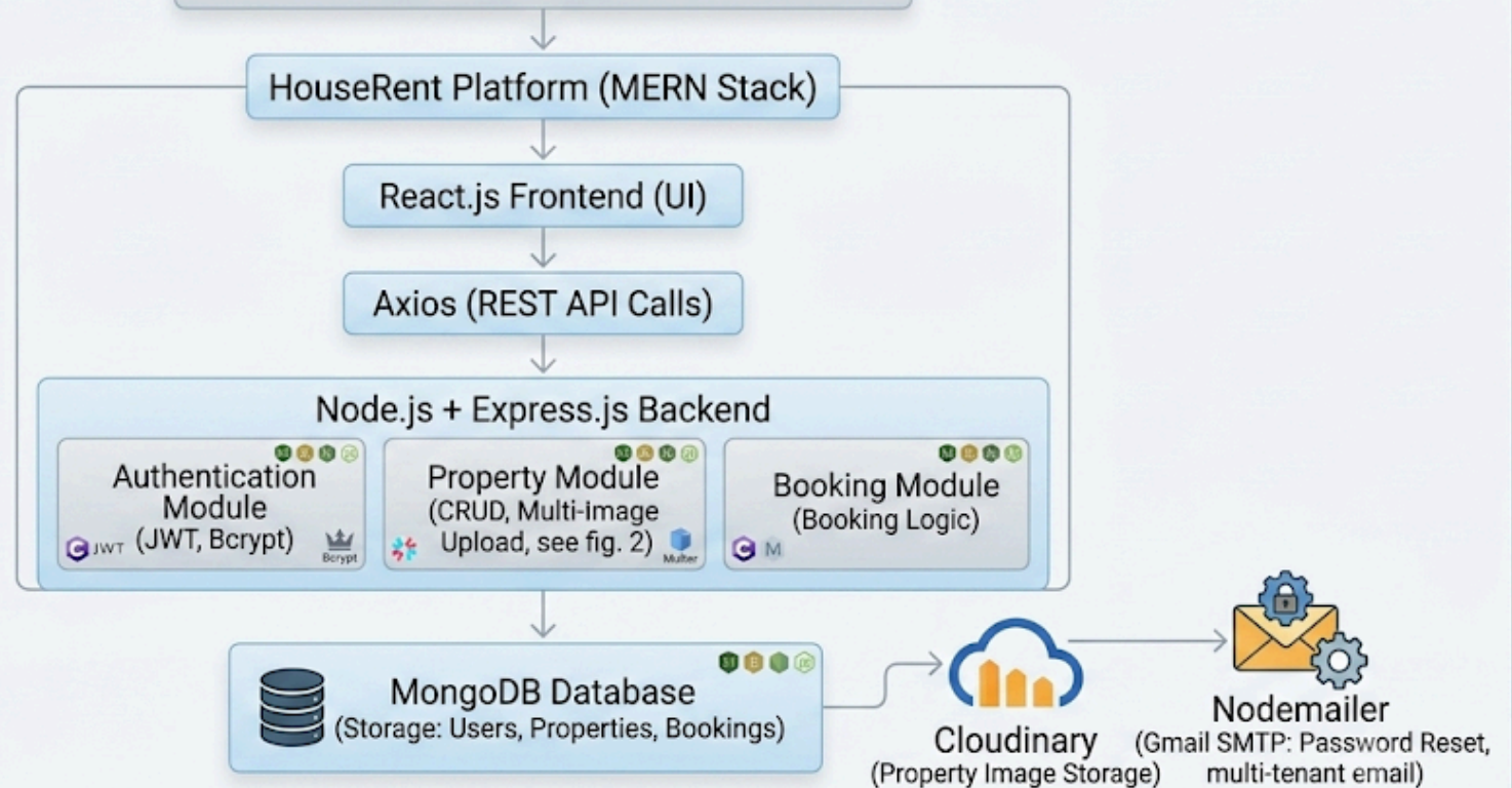
Figure 1: High-Level Platform Architecture
