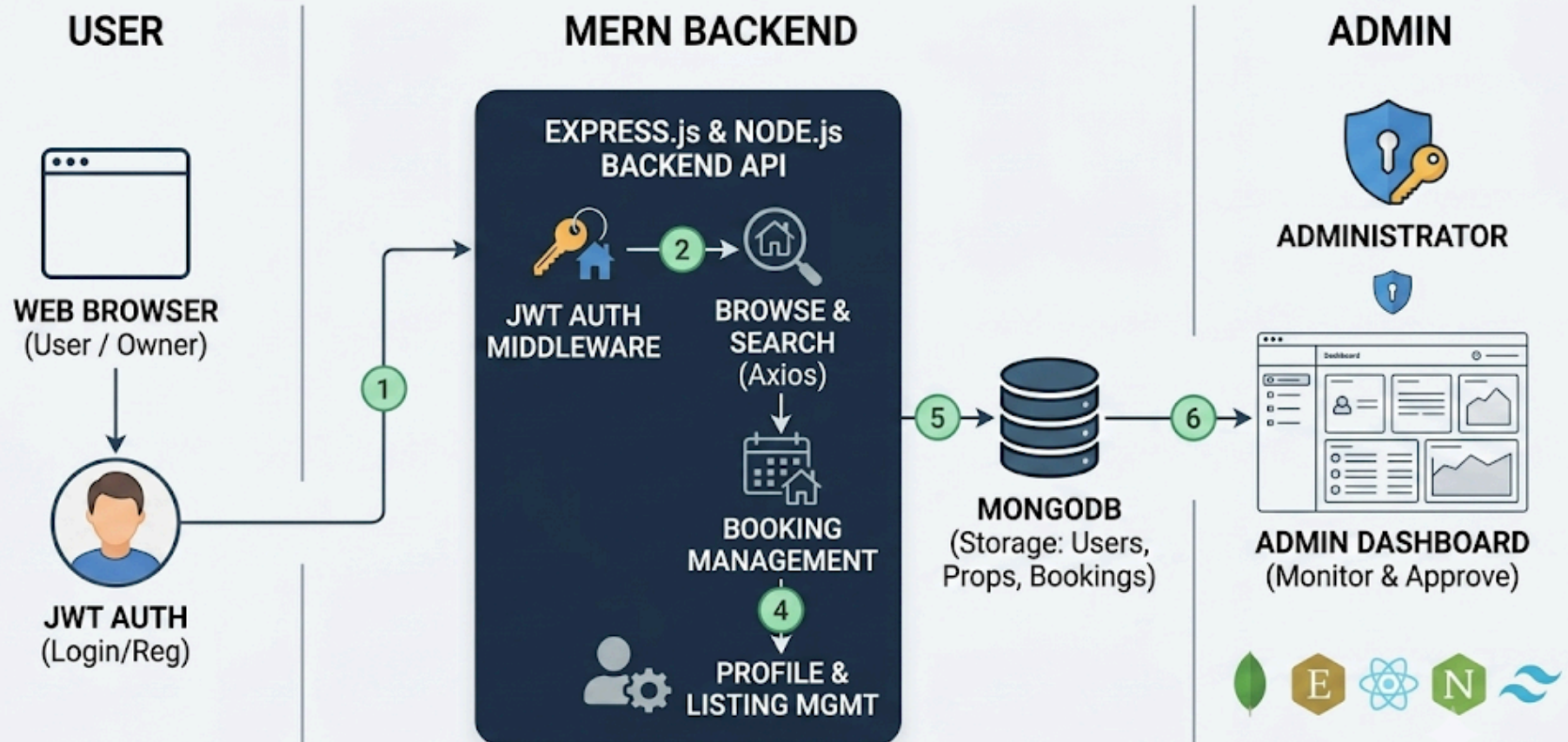
Figure 1: Architecture and data flow of the HouseRental platform
